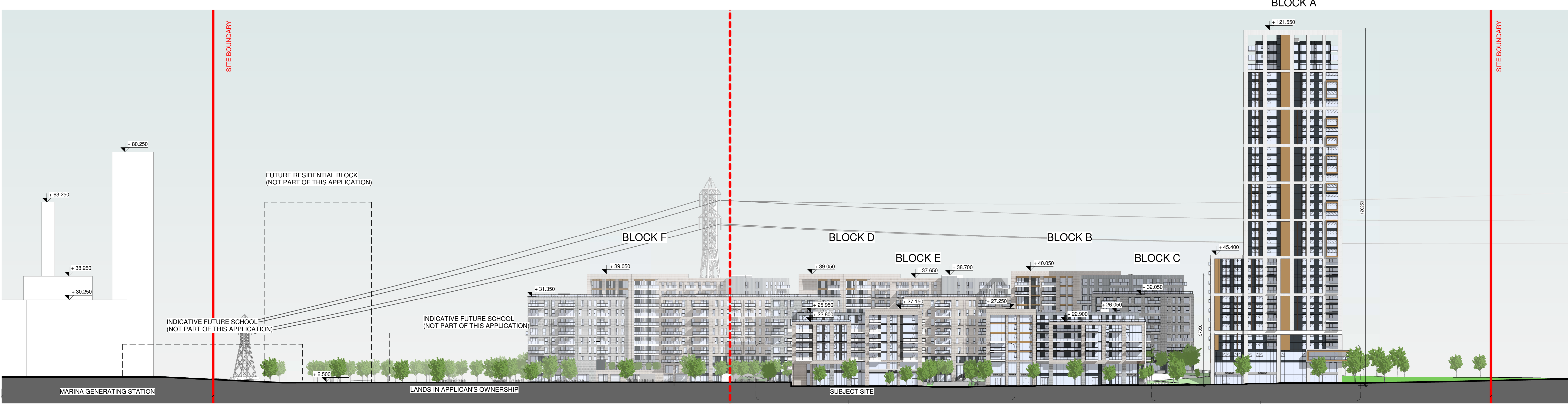
1 PROPOSED CONTEXTUAL SITE SECTION D-D 1:500
